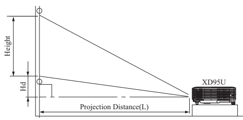
Screen size chart (4:3 aspect ratio)
